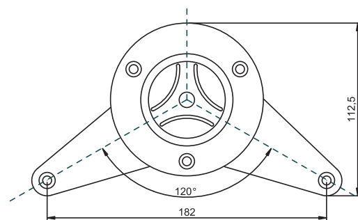
Piastra in alluminio pressofuso attacco ortogonale 90° Aluminium alloy plate for 90° orthogonal connection
