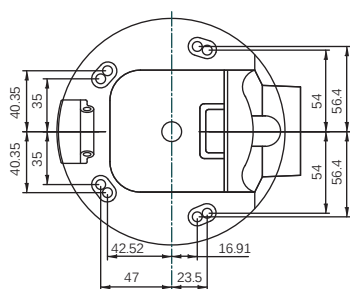
Piastra in nylon per gamba pieghevole FLEXO Nylon plate for folding leg FLEXO
